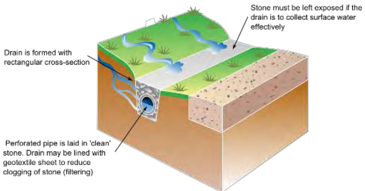
French drain
